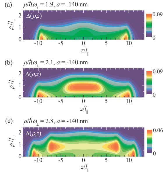
FIG. 3. (Color online) Contour plots of the order parameter \Delta(\rho,z) obtained for a = -140 nm (at T = 0 ) below the resonance at \mu/\hbar\omega_{\perp} = 1.9 (a), in the vicinity of the resonance at \mu/\hbar\omega_{\perp} = 2.1 (b) and far beyond it at \mu/\hbar\omega_{\perp} = 2.8 (c).
