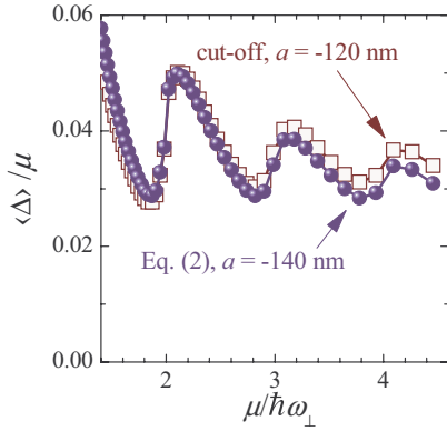
FIG. 5. (Color online) The averaged energy gap \langle \Delta \rangle (in units of \mu ) versus \mu/\hbar\omega_{\perp} : squares are results for a = -120 nm calculated with the Bruun-Heiselberg cutoff |\lambda_v| < \mu ; circles are the data from Fig. 1(a).
