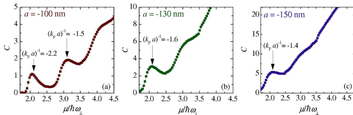
Figure 1: The longitudinal contact intensity as function of the chemical potential (in units of the transverse trapping energy) for the cigar-shaped superfluid Fermi gas of {}^6\text{Li} : (a) for the scattering length a = -100 nm; (b) for a = -130 nm; and (c) a = -150 nm. Each time when the ratio of the chemical potential to the transverse confinement energy approaches an integer number, a new single-particle subband touches the chemical potential and the atypical BCS-BEC crossover is approached. In calculations we increased the chemical potential whereas the parameters of the trap were kept constant.
