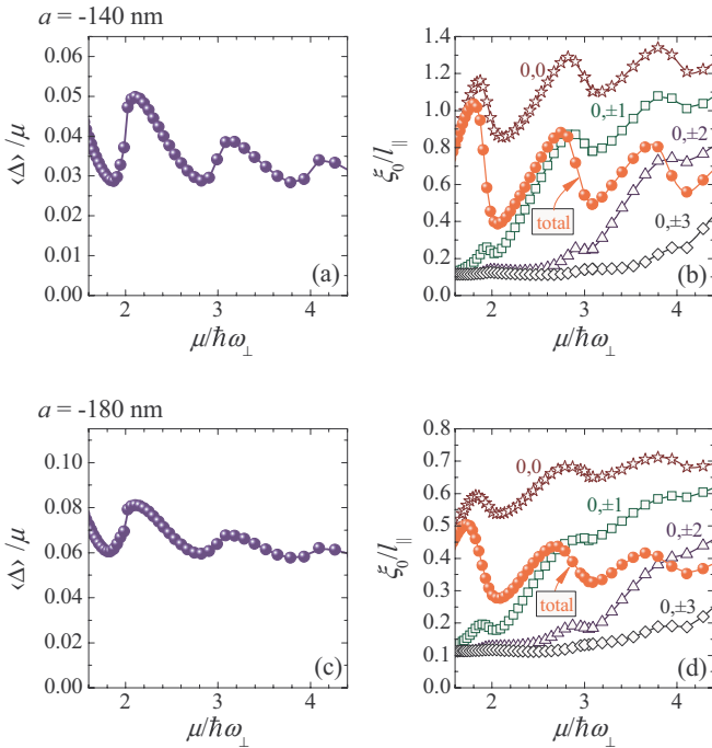
FIG. 1. (Color online) Panels (a) and (c) demonstrate the QS oscillations of the averaged pairing gap \langle\Delta\rangle for scattering lengths a = -140 and -180 nm, respectively. Panels (b) and (d) show the corresponding changes in the longitudinal fermionic-pair size \xi_0 [see Eq. (5)] and the subband fermionic-pair size \xi_0^{(nm)} for subbands (n,m) = (0,0), (0,\pm 1) , and (0,\pm 2) .
