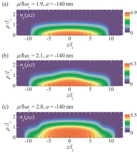
FIG. 4. (Color online) Contour plots of the single-particle density n_p(\rho, z) (given in units of 10^{12} \text{ cm}^{-3} ) calculated for the same parameters as in Figs. 3(a)–3(c), respectively.
