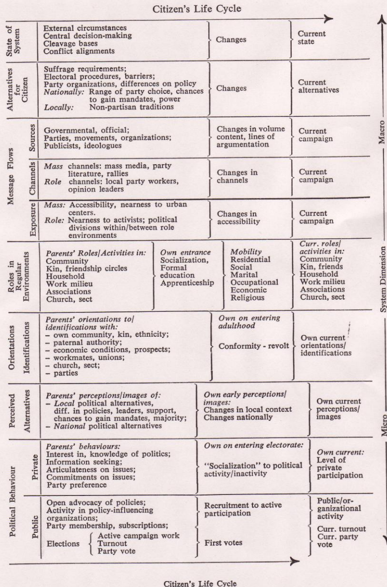
Fig. 2. Location Chart for Variables in Election Research
